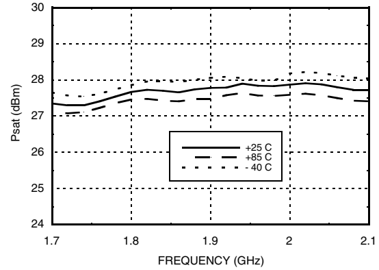
Psat vs. Temperature @ 1900 MHz
