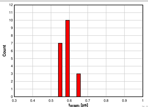
Figure 7-23. Manual Reset Pulse Width Histogram for TPS3823A-33 Devices at 125°C (Unit Count = 20)
