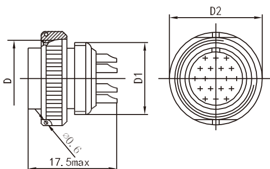
PPC3 Cable socket (female) without tail (PPC3-XXX-0)
