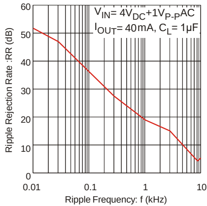
Figure 9: Ripple Rejection Rate
