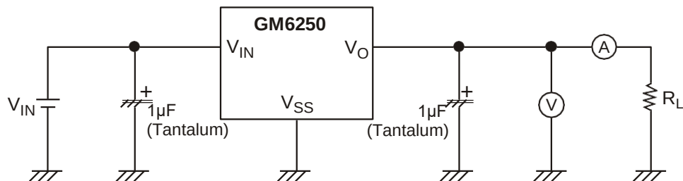
Circuit 1
