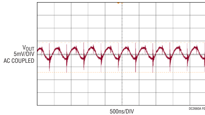
Figure 7. LT8646S Demo Circuit DC2660A Output Voltage Ripple (12V Input, I_{OUT} = 8A , Full BW)
