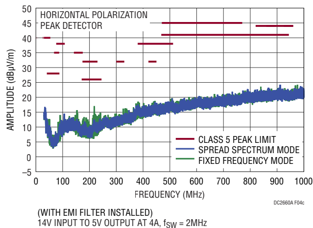
Figure 4. LT8646S Demo Circuit DC2660A EMI Performance (14V Input from VEMI, with EMI filter, I_{OUT} = 4\text{A} )
