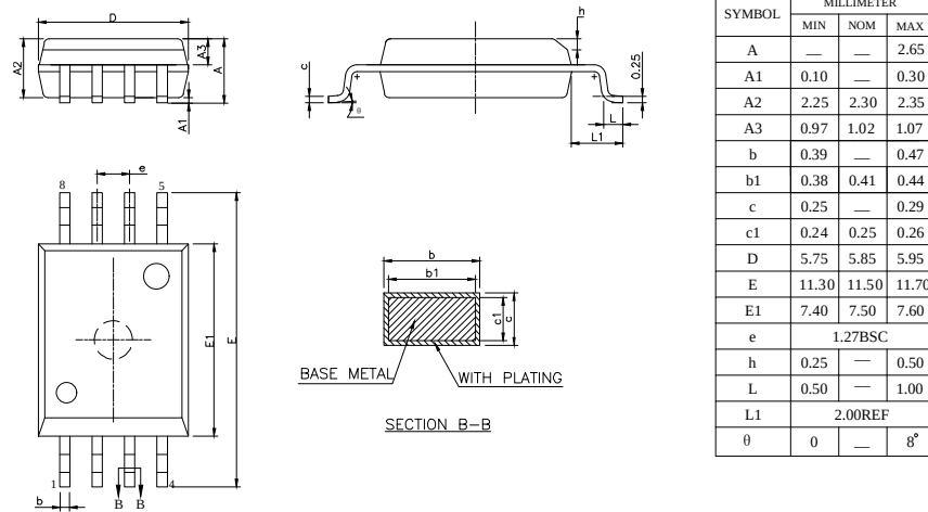
Figure 25. Outline Package
