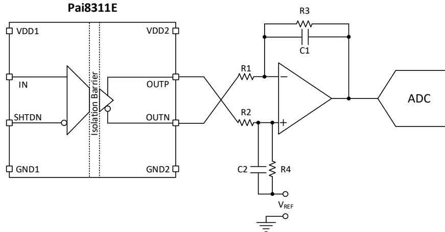
Figure 24. Connecting the Pai8311E Output to a Single-Ended Input ADC
