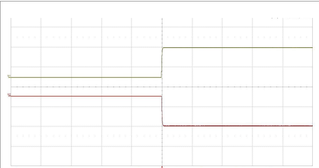
Start-up enabled by connecting V_I at: T_{P1} = +25^\circ\text{C} , V_I = 48\text{ V} , I_O = \pm 0.5\text{ A} resistive load. Top trace: output1 voltage (10 V/div.). Bottom trace: output2 voltage (10 V/div.). Time scale: (200 ms/div.).
