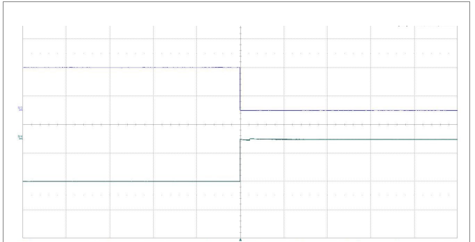
Shut-down enabled by disconnecting V_I at: T_{P1} = +25^\circ\text{C} , V_I = 48\text{ V} , I_O = \pm 0.5\text{ A} resistive load. Top trace: output1 voltage (10 V/div.). Bottom trace: output2 voltage (10 V/div.). Time scale: (200 ms/div.).
