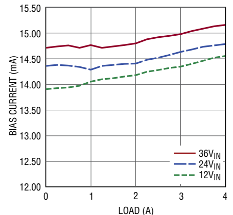
Bias Current vs Load, V_{OUT} = 2.5\text{V}
