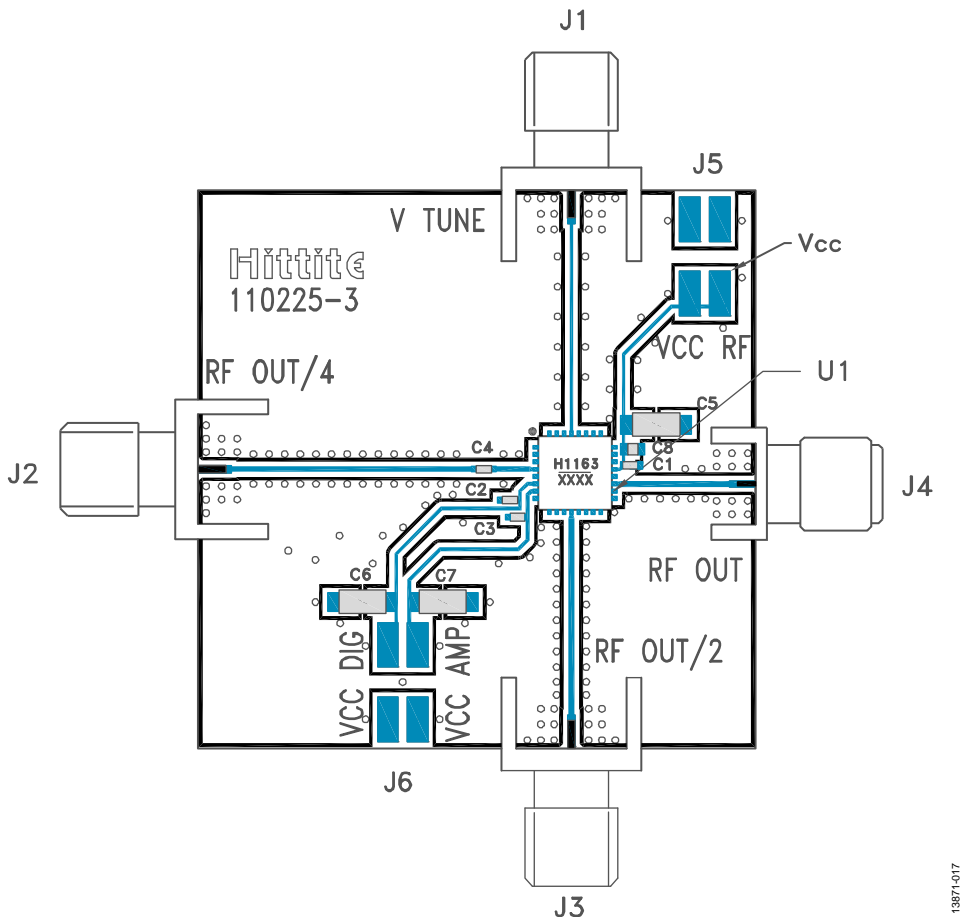
Figure 17. Evaluation PCB
