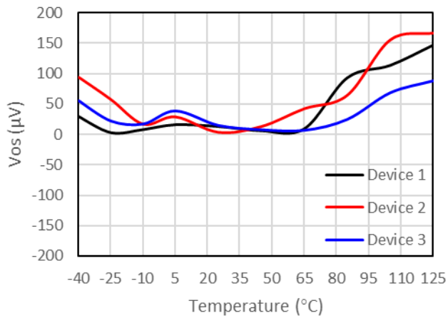
Figure 7-27 Vos vs Temperature (CA-IS1300B25)
